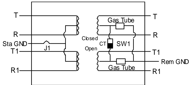
Figure 1: P30116 4-Wire Card Schematic
